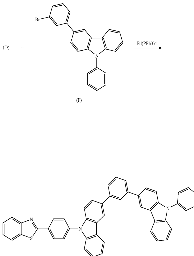
[Reaction Scheme 4]
