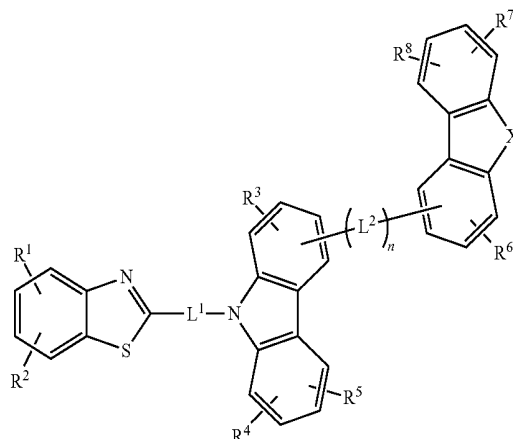
[Chemical Formula 2]
