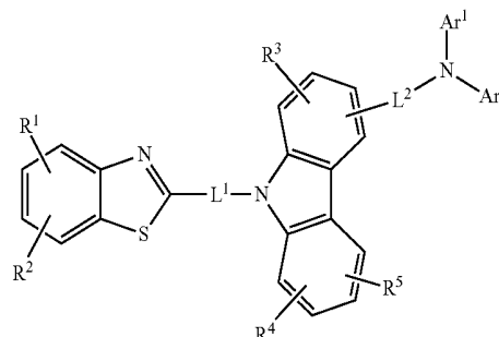
[Chemical Formula 4]
