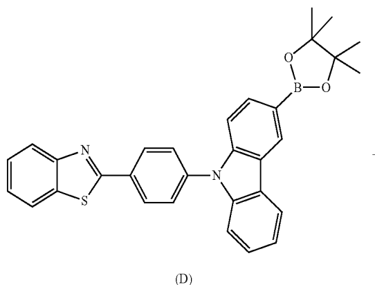
[Reaction Scheme 3]
