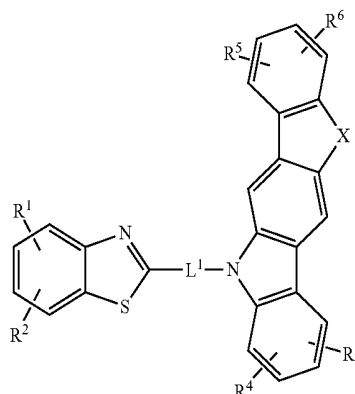
[Chemical Formula 1]
