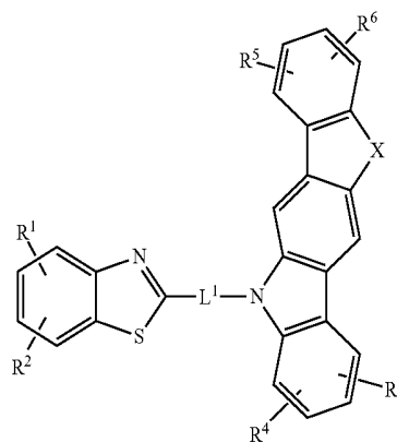
[Chemical Formula 3]
