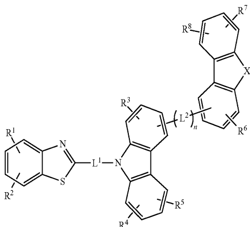
[Chemical Formula 2]
