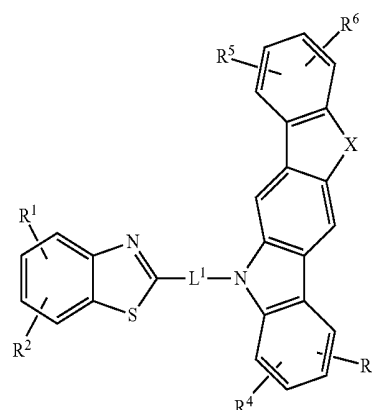
[Chemical Formula 3]
