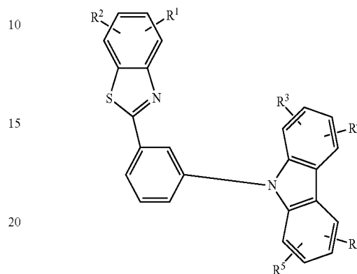
[Chemical Formula 6]
