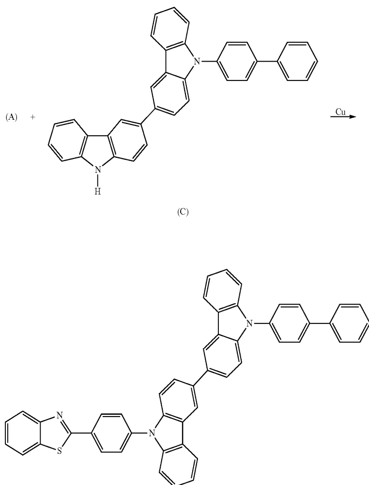
[Reaction Scheme 2]
